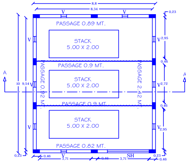
GODOWN PLAN SCALE 1:100
